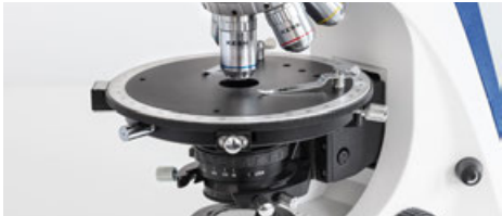
Center-adjustable and turnable polarisation stage
